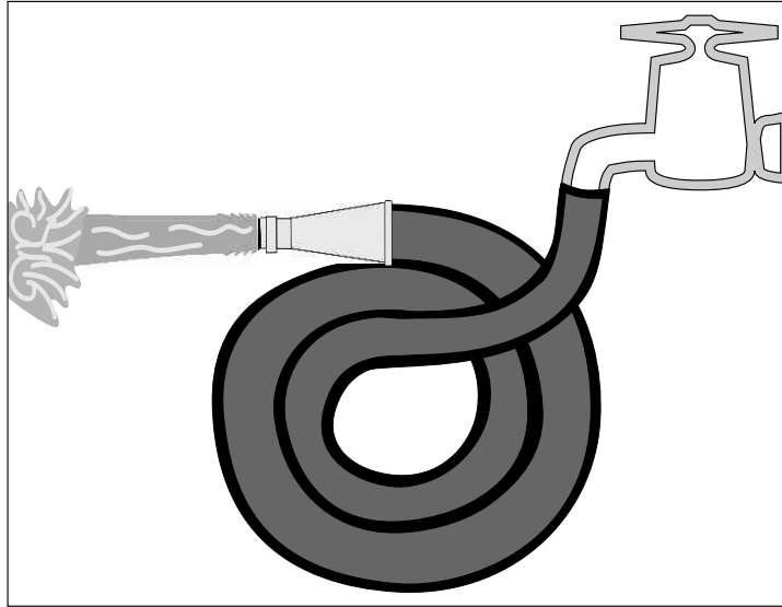
Figure 1.11: Water spurting out of a garden hose
