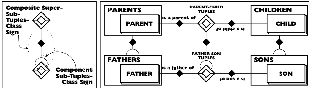
Figure 9.28: Super-sub-tuple-class sign
