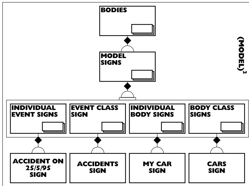
Figure 9.40: (Model) 2 objects
