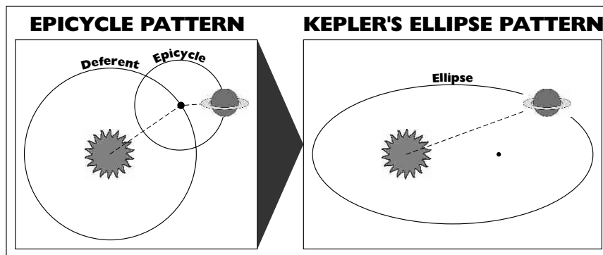
Figure 1.13: Epicyclical and elliptical patterns of planetary motion
