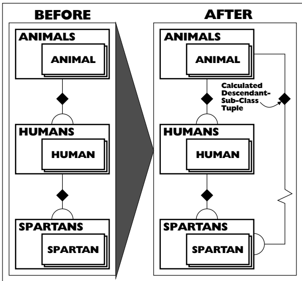
Figure 9.18: Descendant-sub-class calculations
